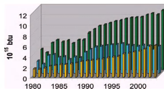
Fig. 1. Iran energy balance net of all trade, 1980–2003. The only nonpetroleum account in Fig. 1 is hydropower, 4.3% of total energy production; thus, this energy balance gives an overview of Iran's petroleum economy. The graph is color-coded as follows: green, production plus imports; blue, exports; gold, domestic consumption.
